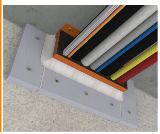
Construct a FyreBOARD Maxilite® wall collar, on one side of the penetration, by fixing 30mm thick x 100mm wide FyreBOARD Maxilite® strips around the three exposed sides of the SuperSTOPPER®. Fix FyreBOARD Maxilite® with 10g x 60mm plasterboard screws at 150mm centres and make certain that FyreBOARD Maxilite® is fixed flush with the wall opening (Trafalgar Fire strongly recommends this step is undertaken by a Trafalgar approved SuperSTOPPER® Certification Partner).
