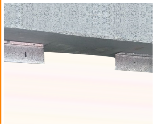
Install the Hebel® wall's fixing angles on either side of the SuperSTOPPER®
