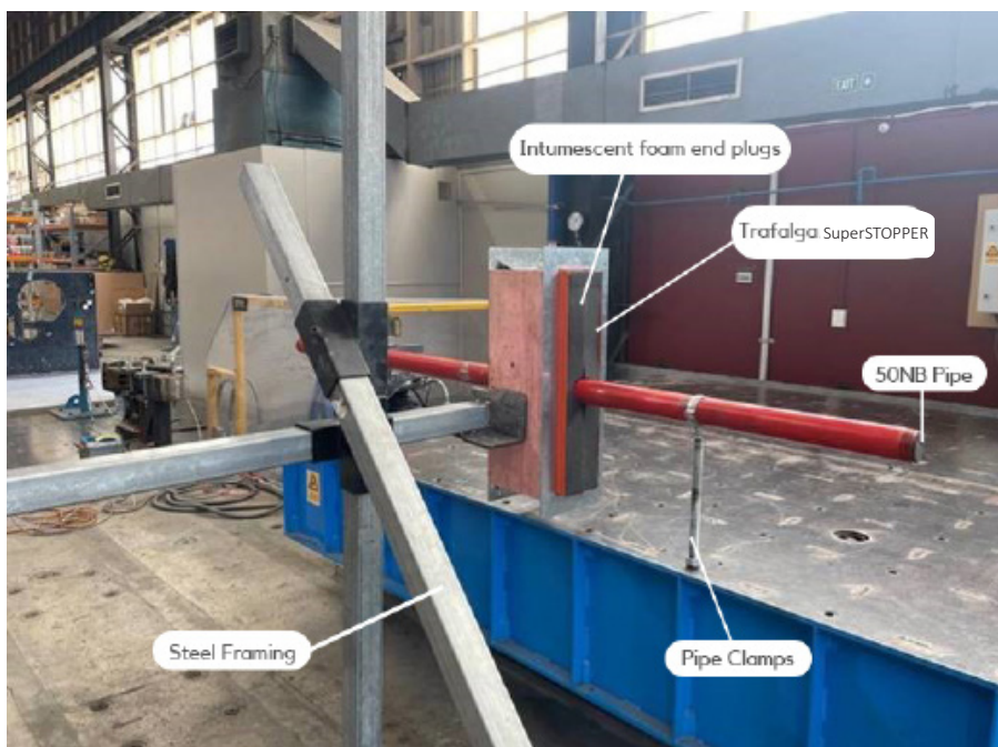
Shake-table test setup of Trafalgar SuperSTOPPER MAXI
